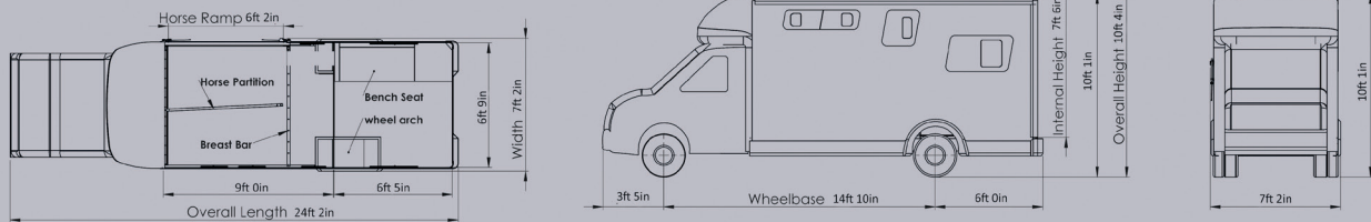
Vision layout
